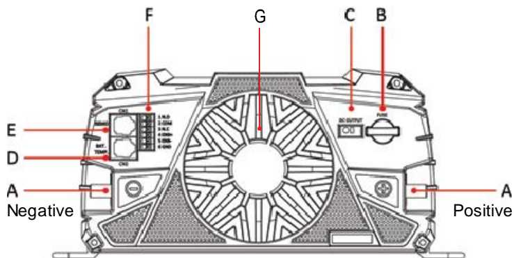
Figure 5: DC side
