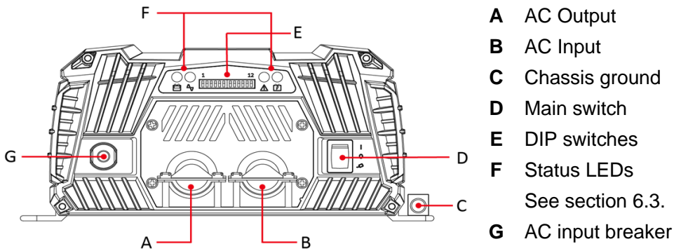
Figure 3: AC side – exterior
