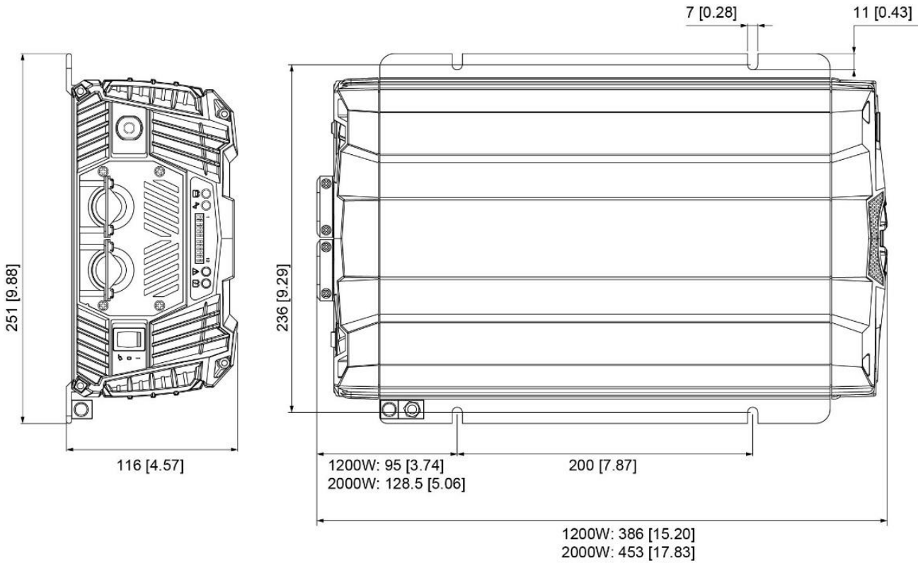
Figure 2: Dimensions PowerCombi in mm [inch]
