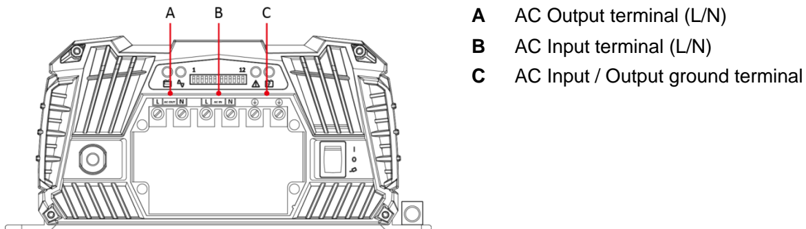
Figure 4: AC side – interior
