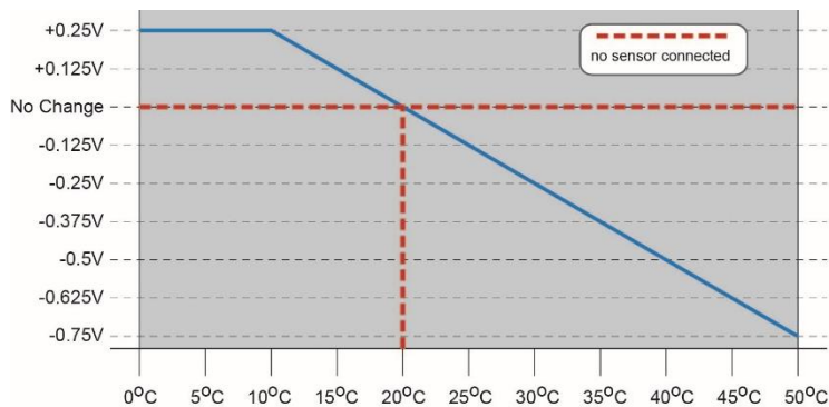
Figure 9 : Temperature compensation using battery temperature sensor
