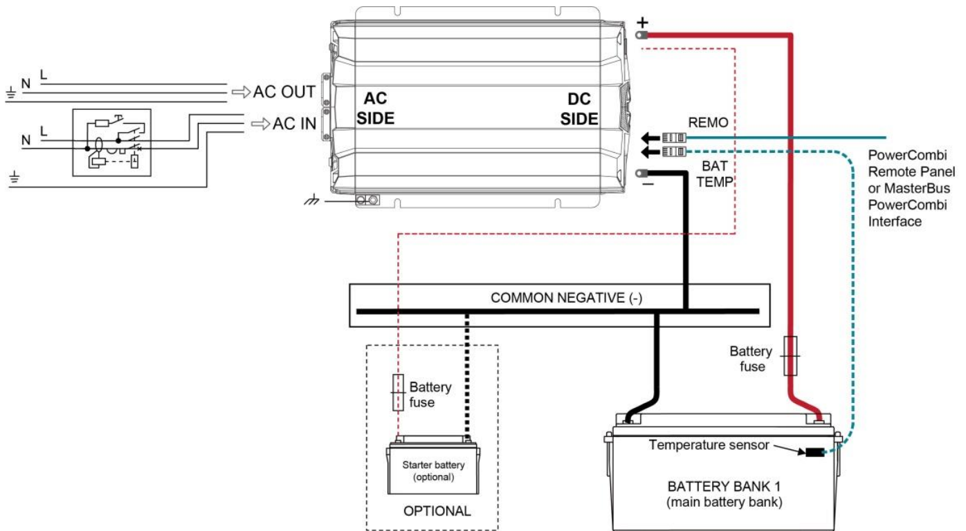
Figure 7: Installation drawing PowerCombi Inverter/Charger
