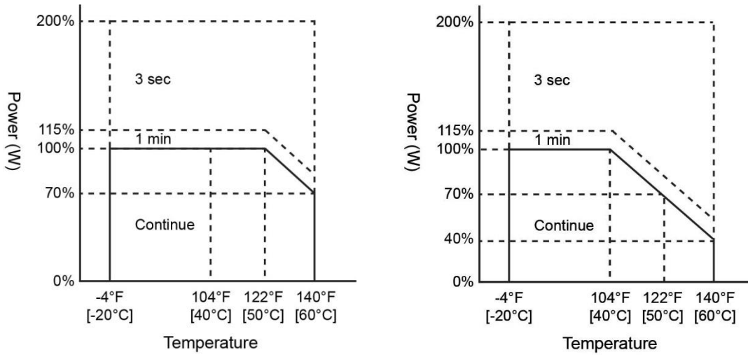
Figure 10 : PowerCombi 1200W (left) and PowerCombi 2000W (right) De-rating Curve
