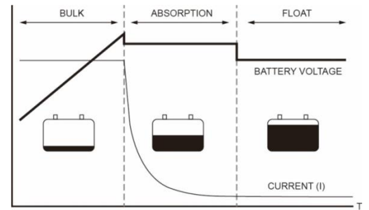
Figure 8: Three step charge system
